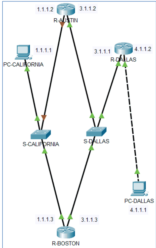
Figure 13.3 Network topology with Fa0/0 interface failure in R-AUSTIN
