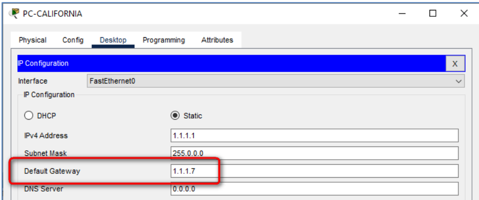
Figure 13.6 Changing the address of the default gateway in PC- CALIFORNIA
